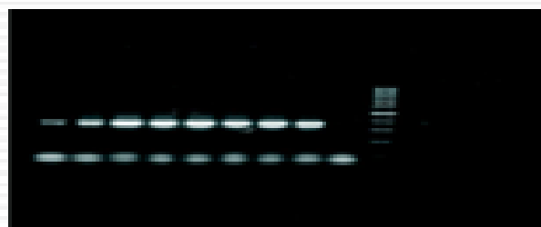
Amplification of Cytb (307bp)
